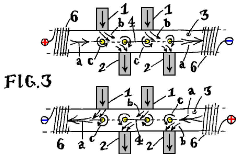
Fig.3 is a schematic diagram of the magnetic action occurring within the generator of Fig.1 and Fig.2 .
